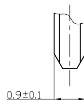
DETAIL OF TERMINALS (10:1)
