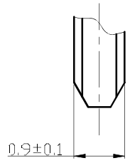
DETAIL OF TERMINALS (10:1)
