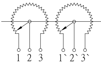
CIRCUIT
