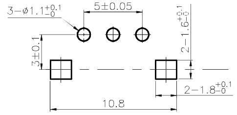
PCB Holes Layout THICKNESS PCB 1.5mm
