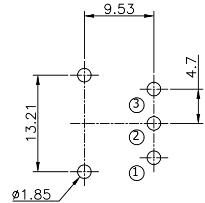
P.C.MOUNTING
