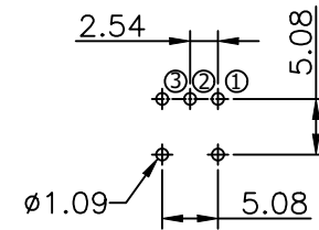
P.C.MOUNTING
