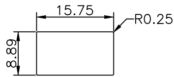
PANEL MOUNTING
