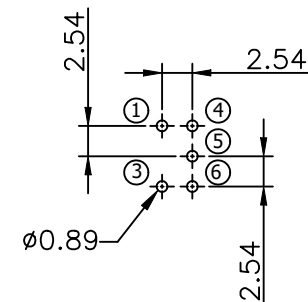
P.C.MOUNTING
