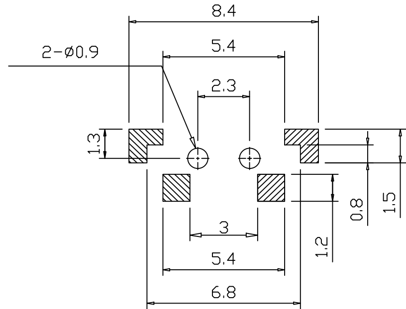
PCB LAYOUT
