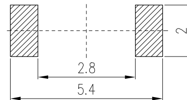
SMD REFLOW PATTERN
